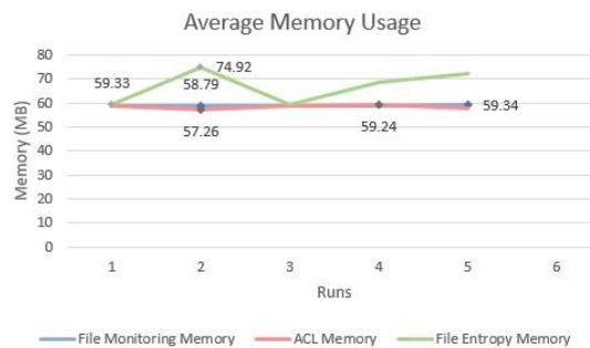
Figure 2: Memory Averages of implementations
